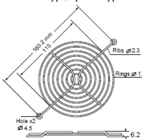
TWG-127-82 for 127mm 2 Rib Type, Special Type
