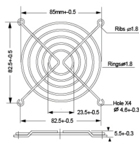
TWG-92 for 92mm Standard Type
