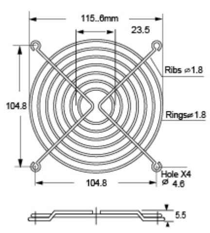
TWG-120-17 for 120mm Standard Type
