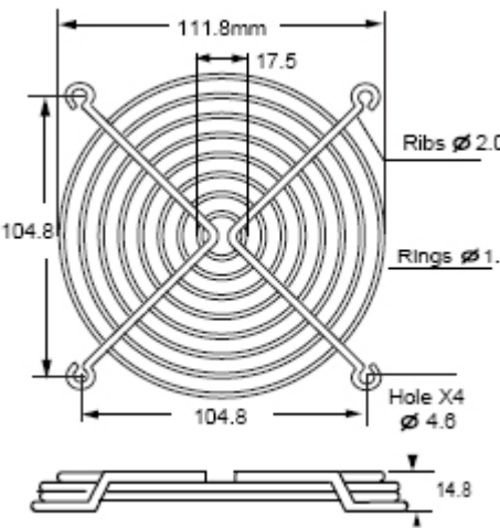
TWG-120-8R2 for 120mm 2 Ring Raised Type, Special Type
