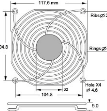
TWG-120-8R3, for 120mm 3 Ring Raised Type, Special Type
