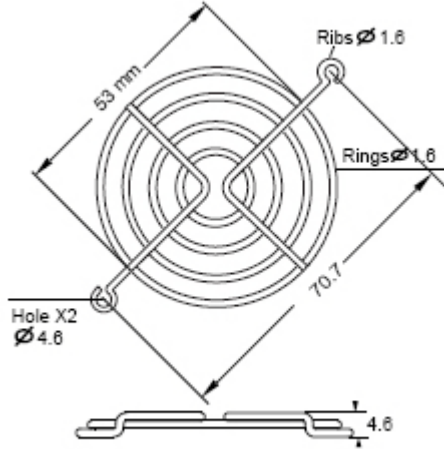
TWG-60 for 60mm 2 Rib Type, Special Type
