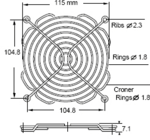
TWG-120-E, for 120mm Fan Special Disk Type
