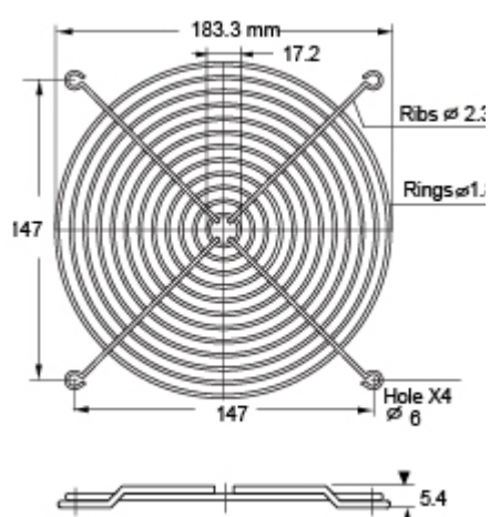
TWG-200 for 200mm Fan Standard Type
