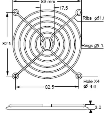
TWG-92F for 92mm Flat Type, Special Type
