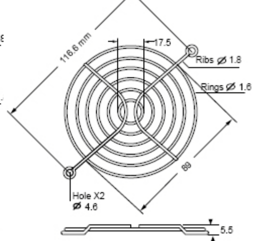
TWG-92-2, for 92mm 2 Rib Type, Special Type
