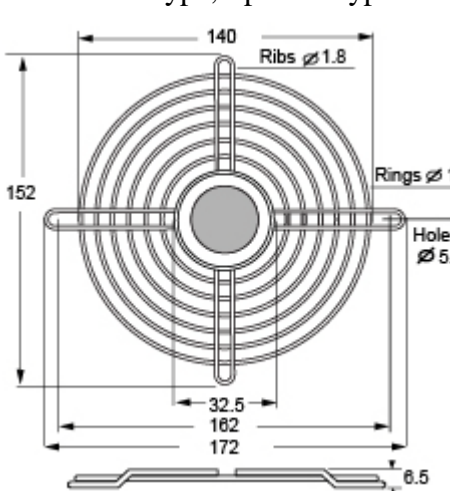
TWG-172-7DU for 172mm Center Disk Type, Special Type
