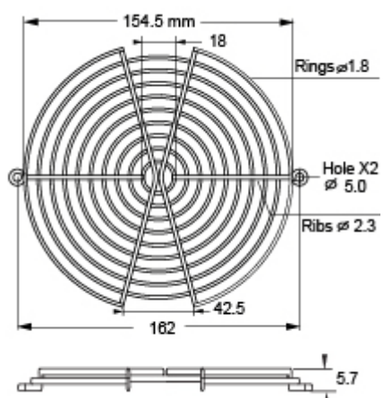
TWG-172-10H for 172mm Standard Type
