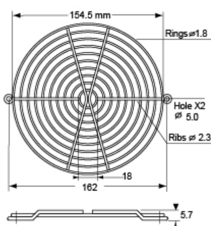
TWG-172-10HA for 172mm Standard Type
