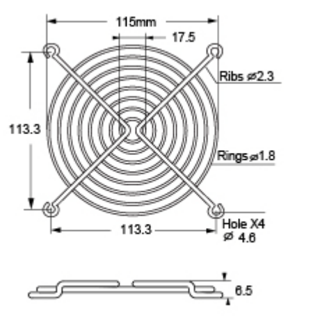
TWG-127 for 127mm Standard Type
