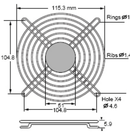
TWG-120-8R2 for 120mm 2 Ring Raised Type, Special Type
