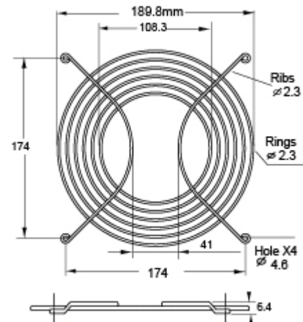
TWG-205-6, for 205mm Standard Type
