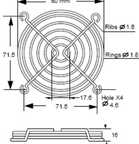
TWG80-2 for 80mm 2 Ring Raised Type, Special Type
