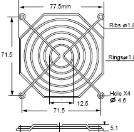
TWG80-1 for 80mm Special Type
