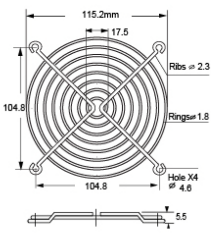
TWG-120-5 for 120mm
