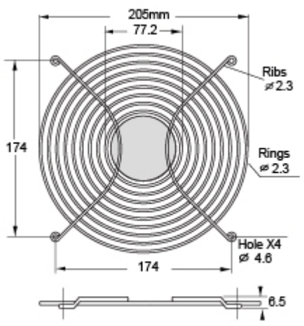
TWG-205 for 205mm Standard Type
