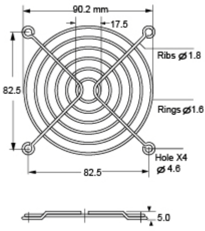
TWG-92-1 for 92mm Standard Type
