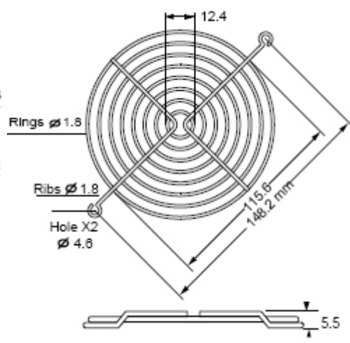
TWG-120-2 for 120mm 2 Rib Type, Special Type
