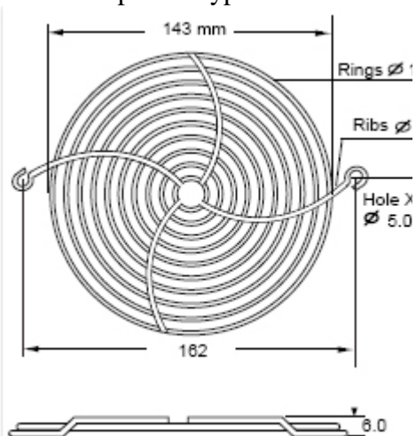
TWG-172-10S for 172mm Fan Special Type
