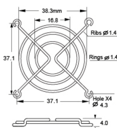
TWG-45 for 45mm Special Type
