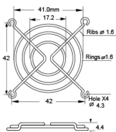
TWG-50 for 50mm Standard Type
