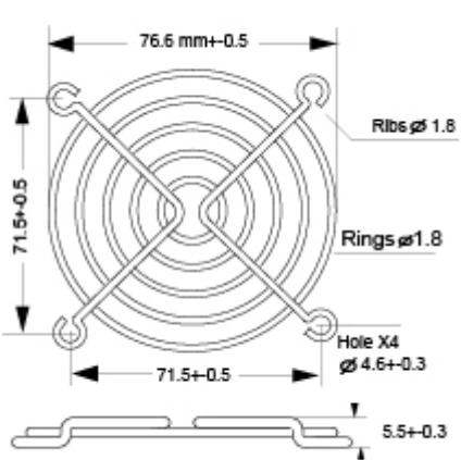
TWG-80 for 80mm Standard Type
