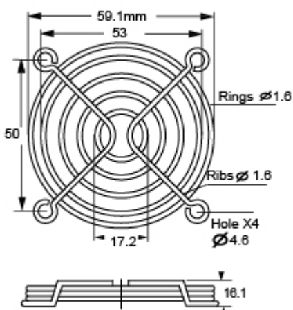
TWG-60 for 60mm 2 Ring Raised Type, Special Type
