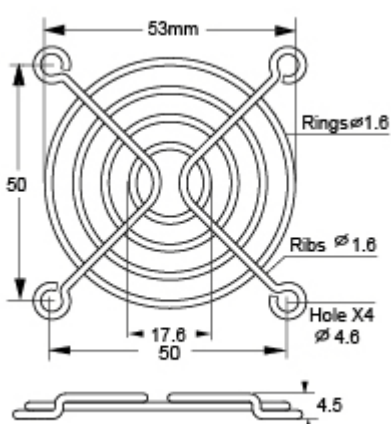
TWG-60 for 60mm Standard Type
