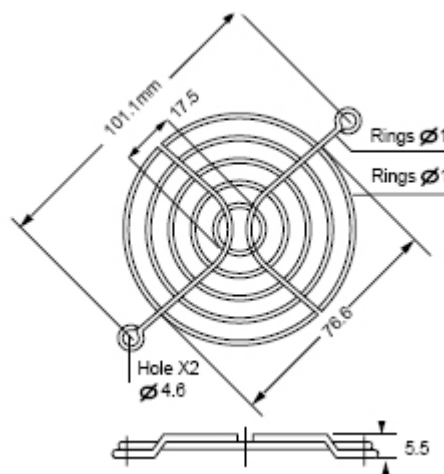
TWG-80-2 for 80mm 2 Rib Type, Special Type
