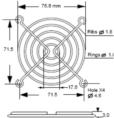
TWG-80F for 80mm Flat Type, Special Type
