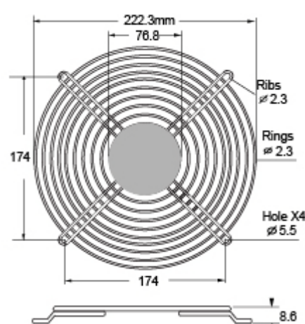
TWG-254-9DU for 254mm Standard Type
