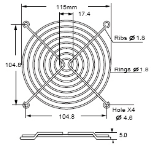
TWG-120-15C for 120mm Special Type
