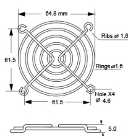
TWG-70 for 70mm Standard Type
