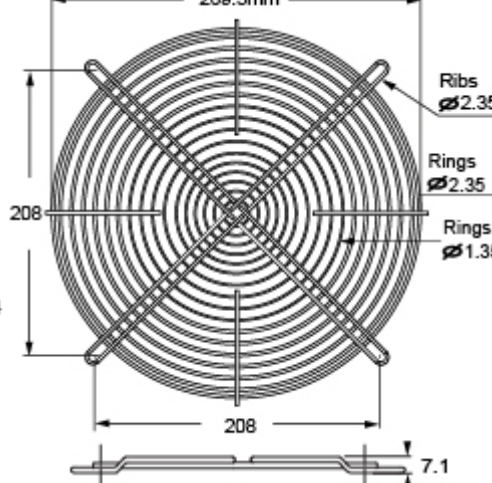
TWG-280 for 280mm Standard Type
